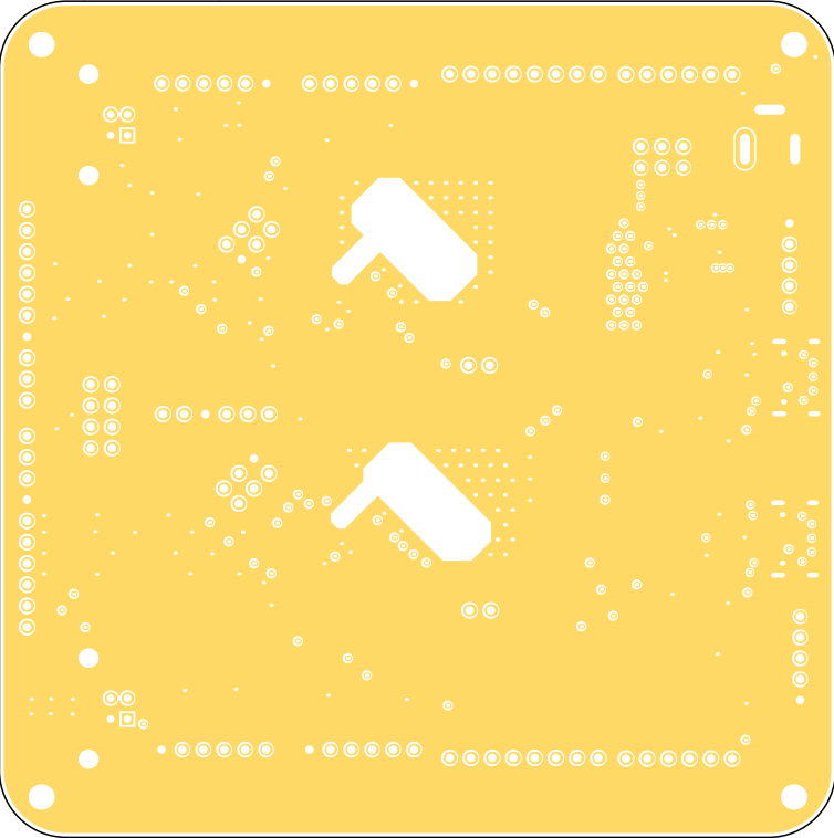
GND (Scale 1:1)
